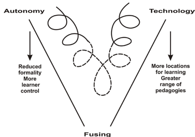
Figure 1. A model of convergence
