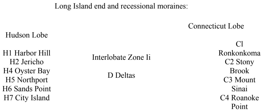
Fig. 1. Late Wisconsinan Moraines of Western Long Island
